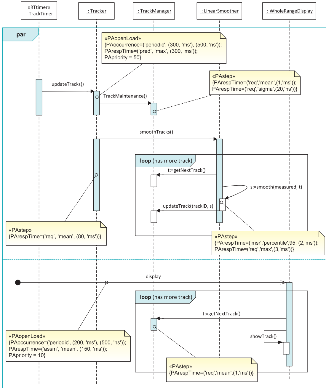
Figure 11.10 Real-time UML: performance annotations.
